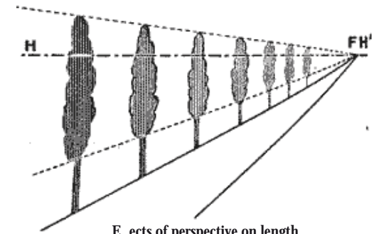
Effects of perspective on length, volume and scale.
