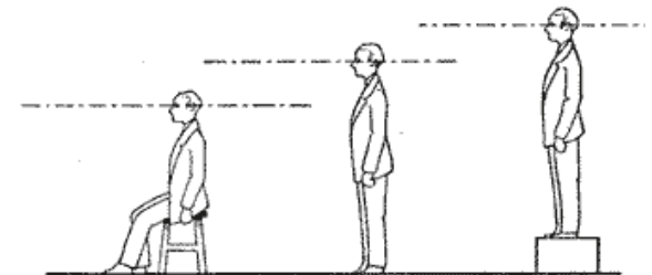
height of the horizon varies with the position of the observer.
